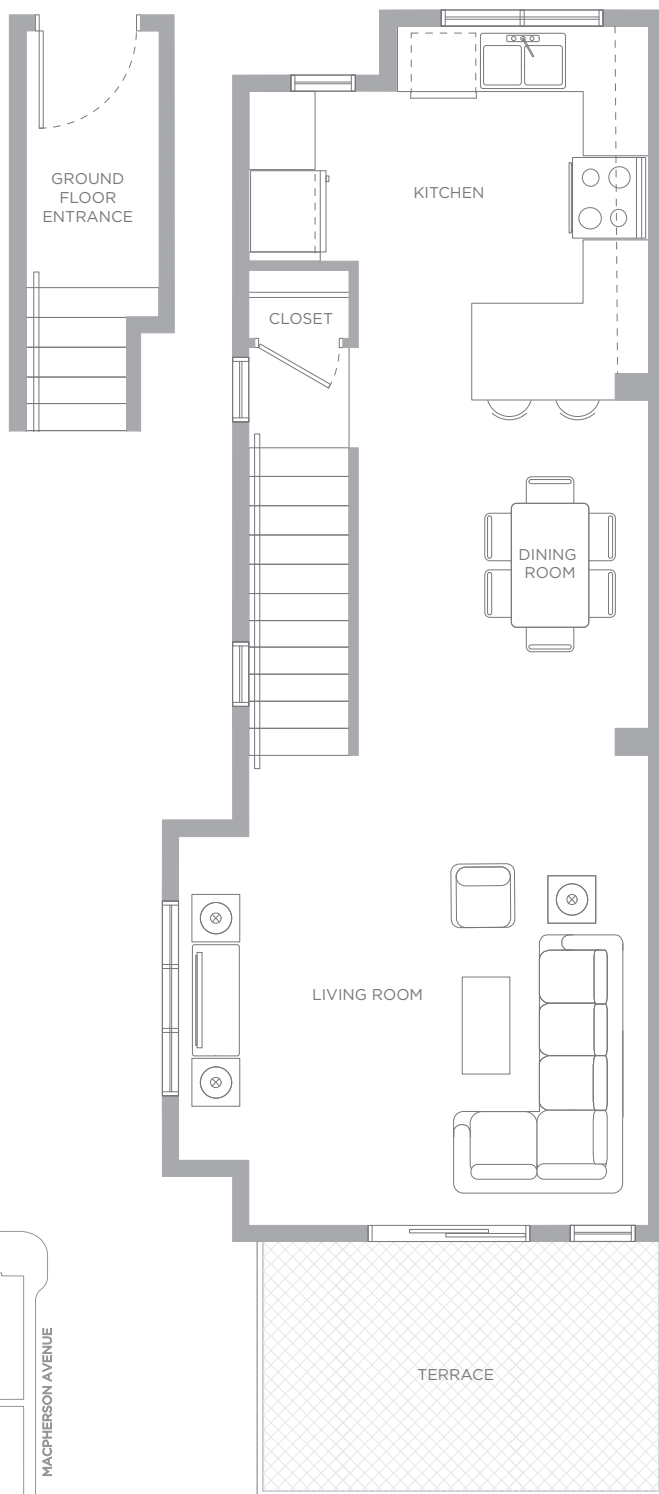
ENTRANCE & FIRST FLOOR | 562 SQ. FT.
